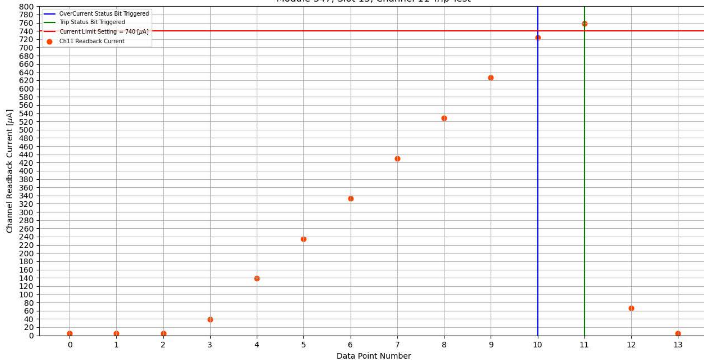
Module 347, Slot 13, Channel 11 Trip Test
