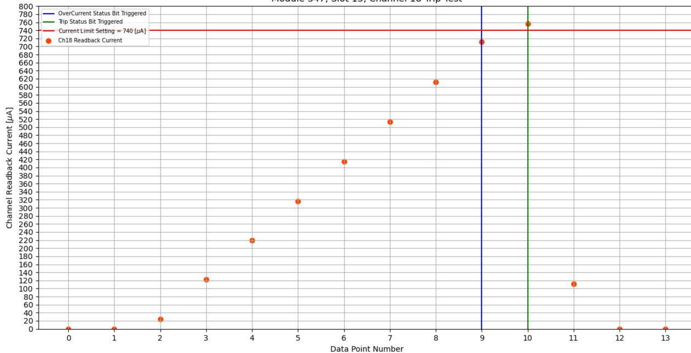
Module 347, Slot 13, Channel 18 Trip Test
