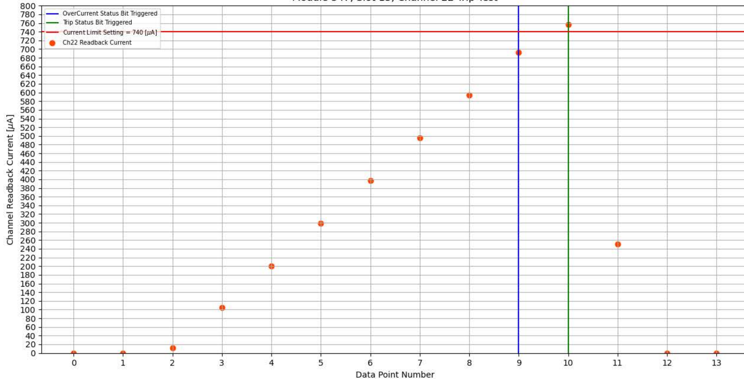
Module 347, Slot 13, Channel 22 Trip Test
