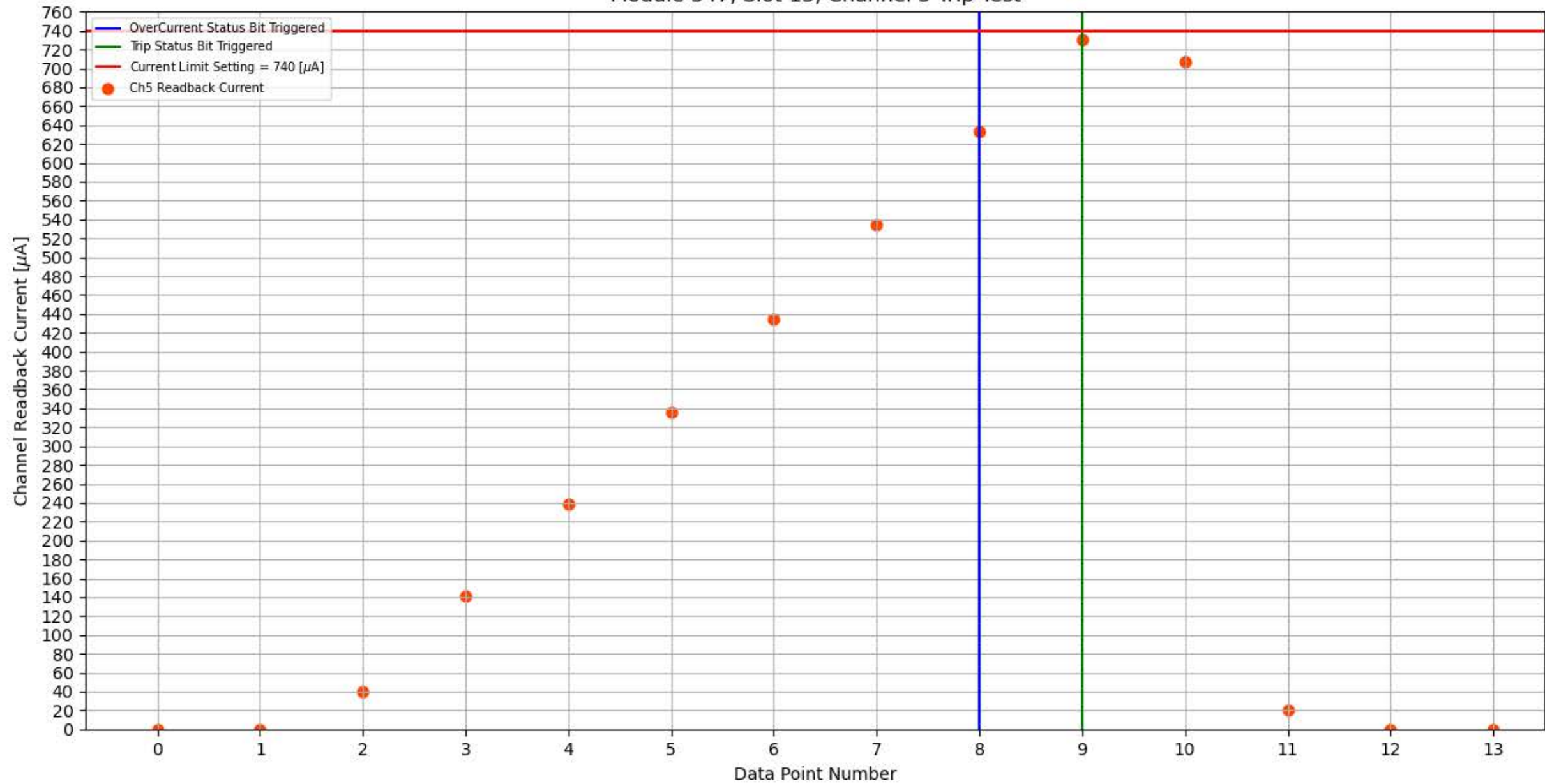
Module 347, Slot 13, Channel 5 Trip Test
