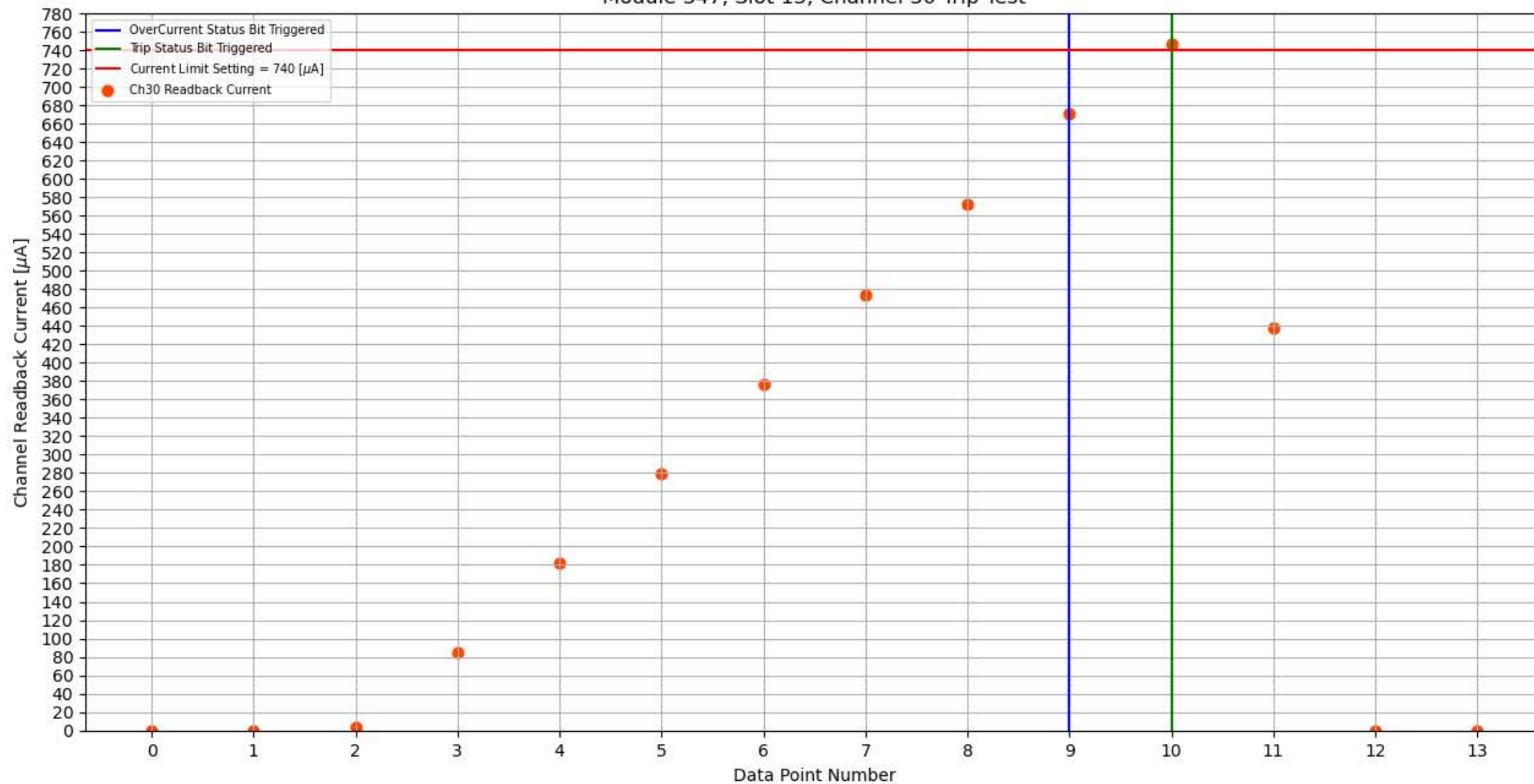
Module 347, Slot 13, Channel 30 Trip Test
