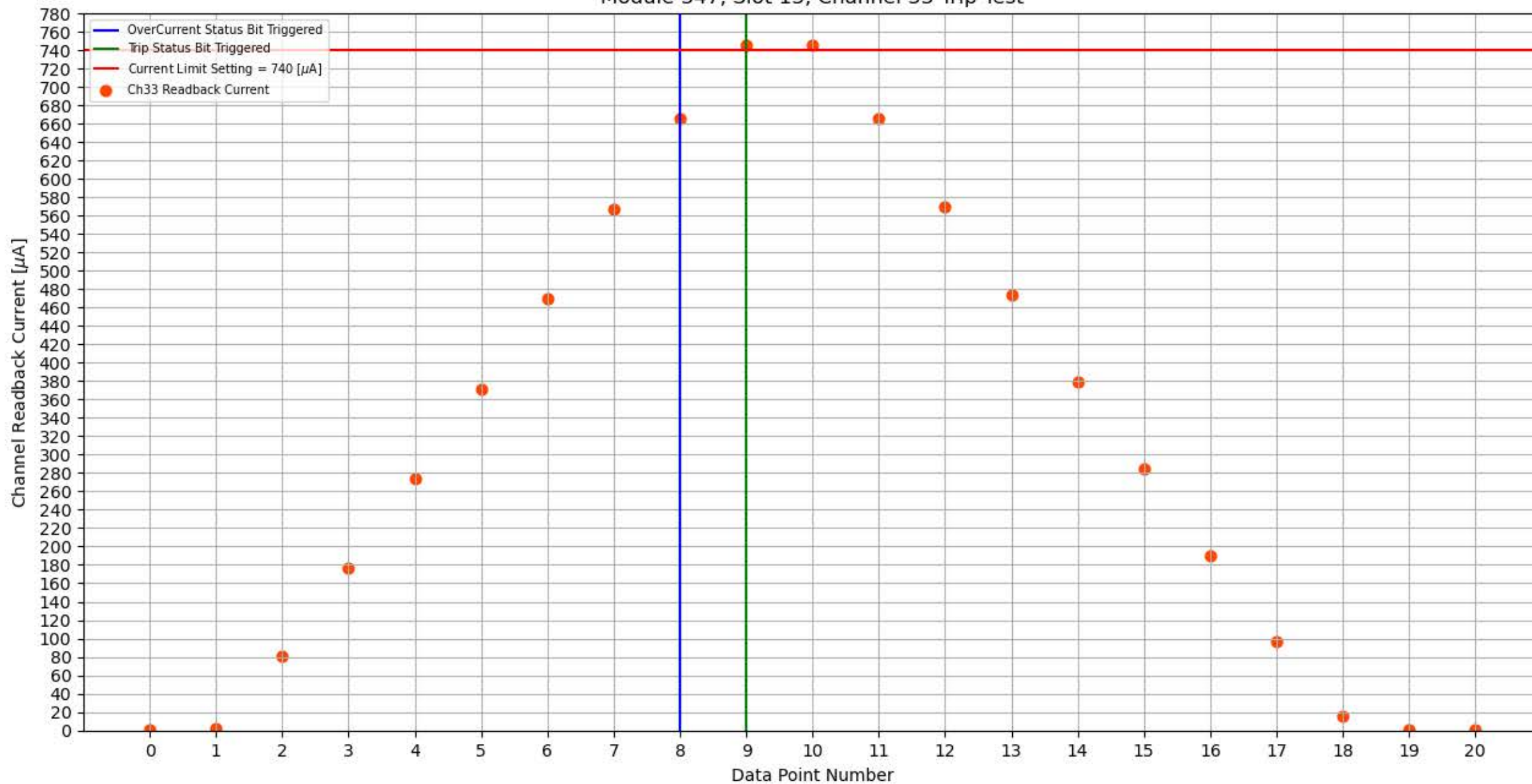
Module 347, Slot 13, Channel 33 Trip Test
