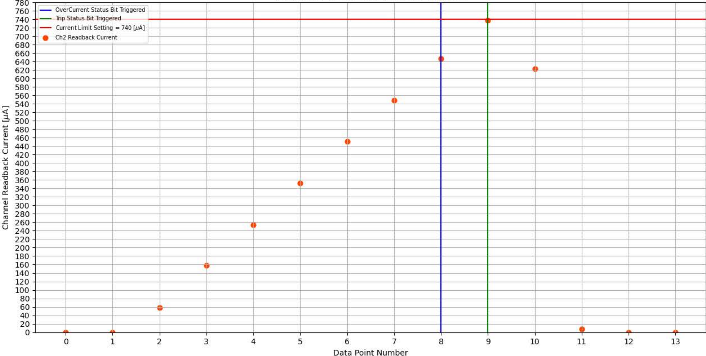
Module 347, Slot 13, Channel 2 Trip Test
