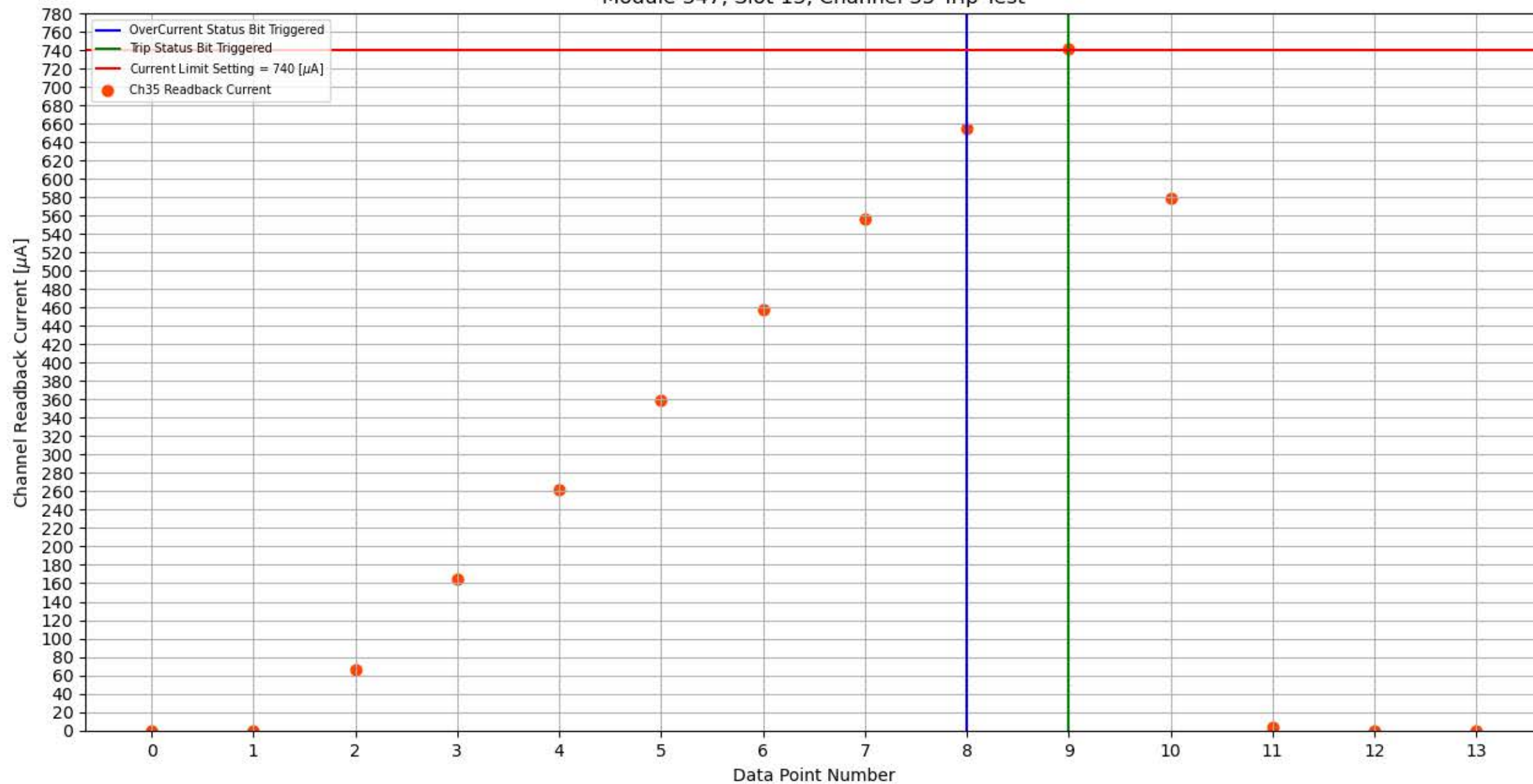
Module 347, Slot 13, Channel 35 Trip Test
