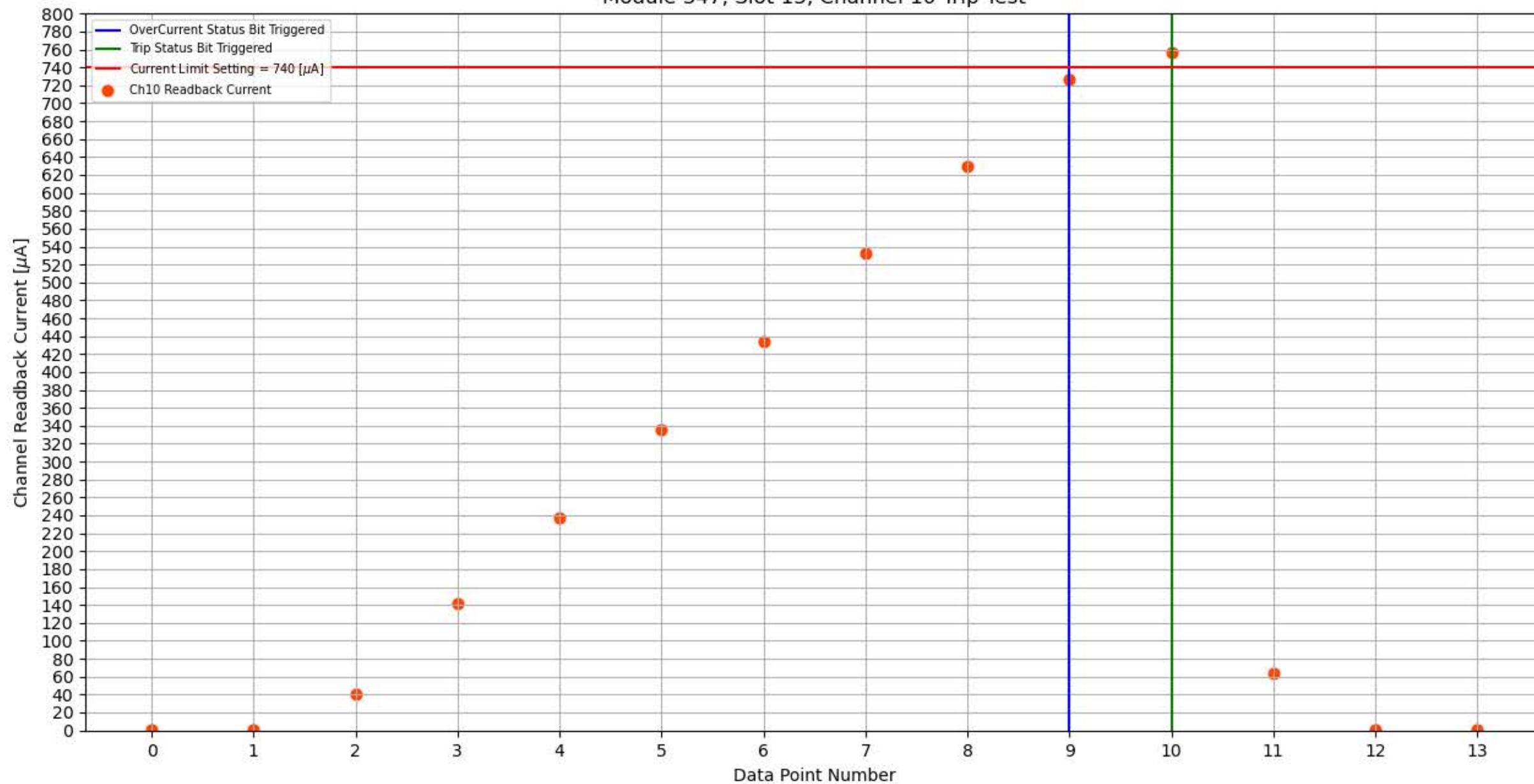
Module 347, Slot 13, Channel 10 Trip Test
