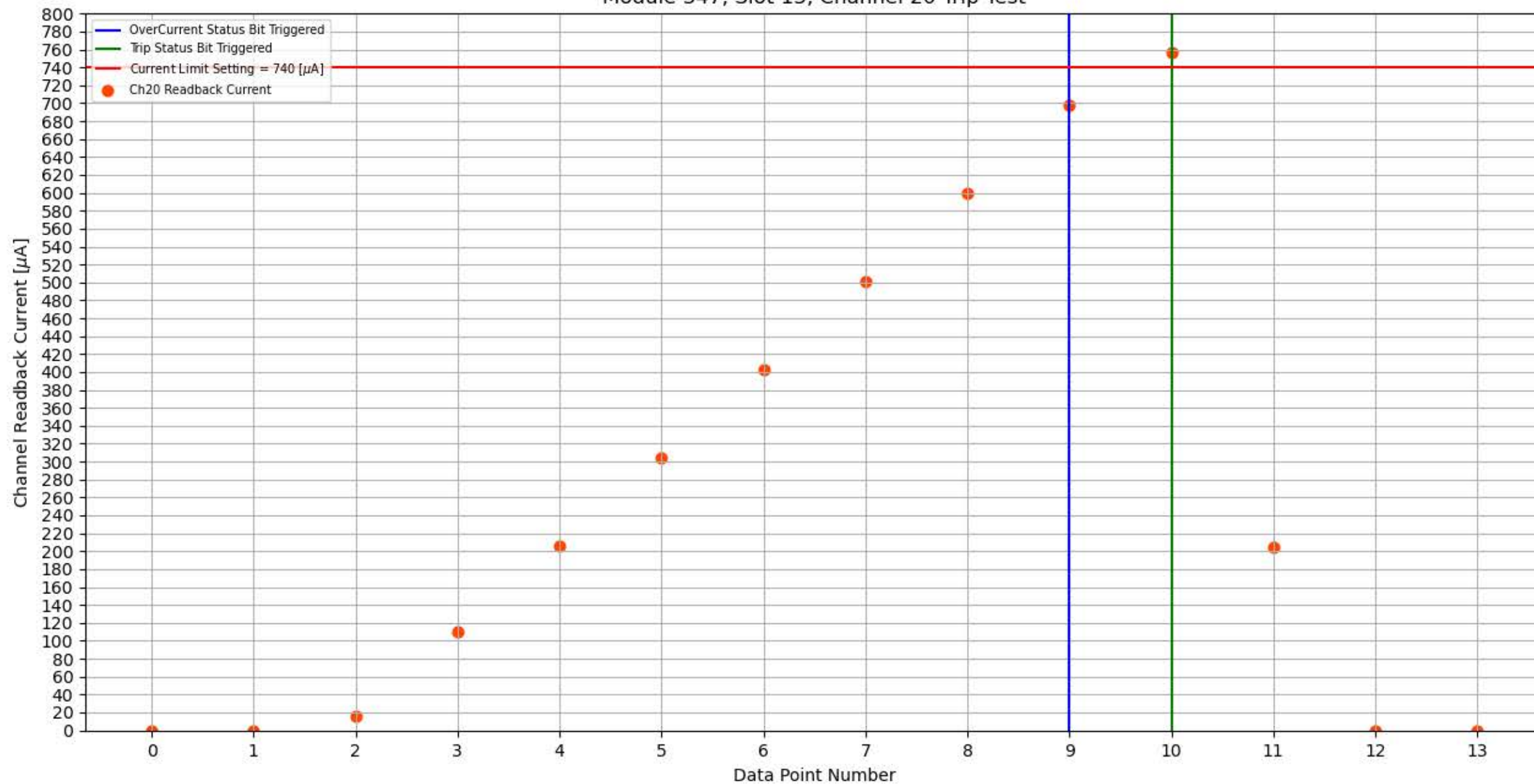
Module 347, Slot 13, Channel 20 Trip Test
