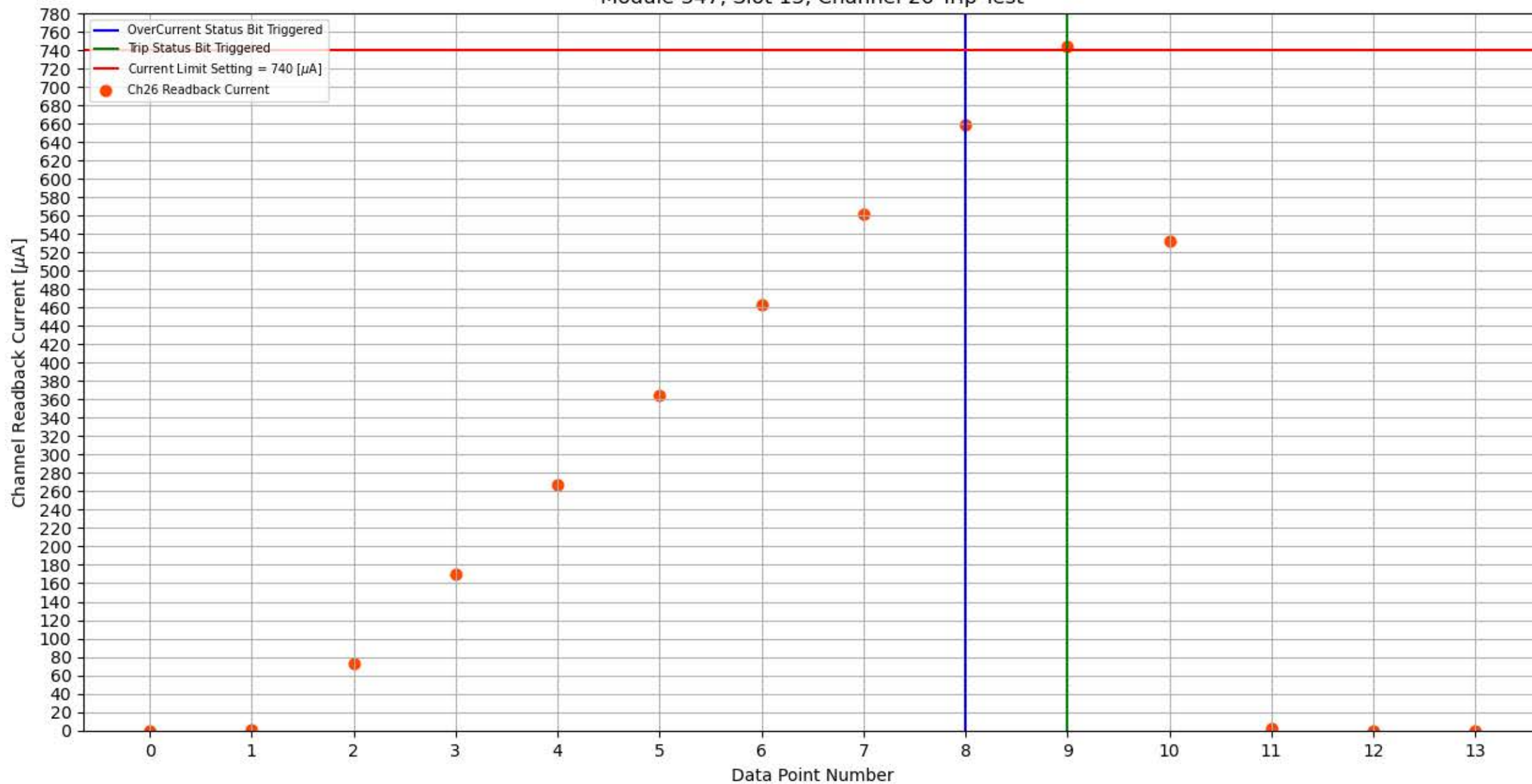
Module 347, Slot 13, Channel 26 Trip Test
