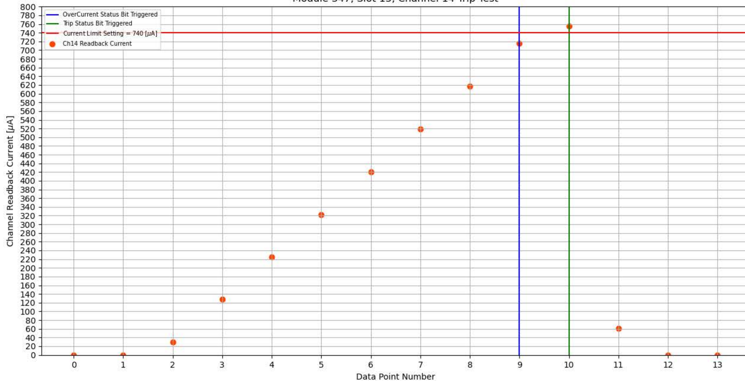
Module 347, Slot 13, Channel 14 Trip Test
