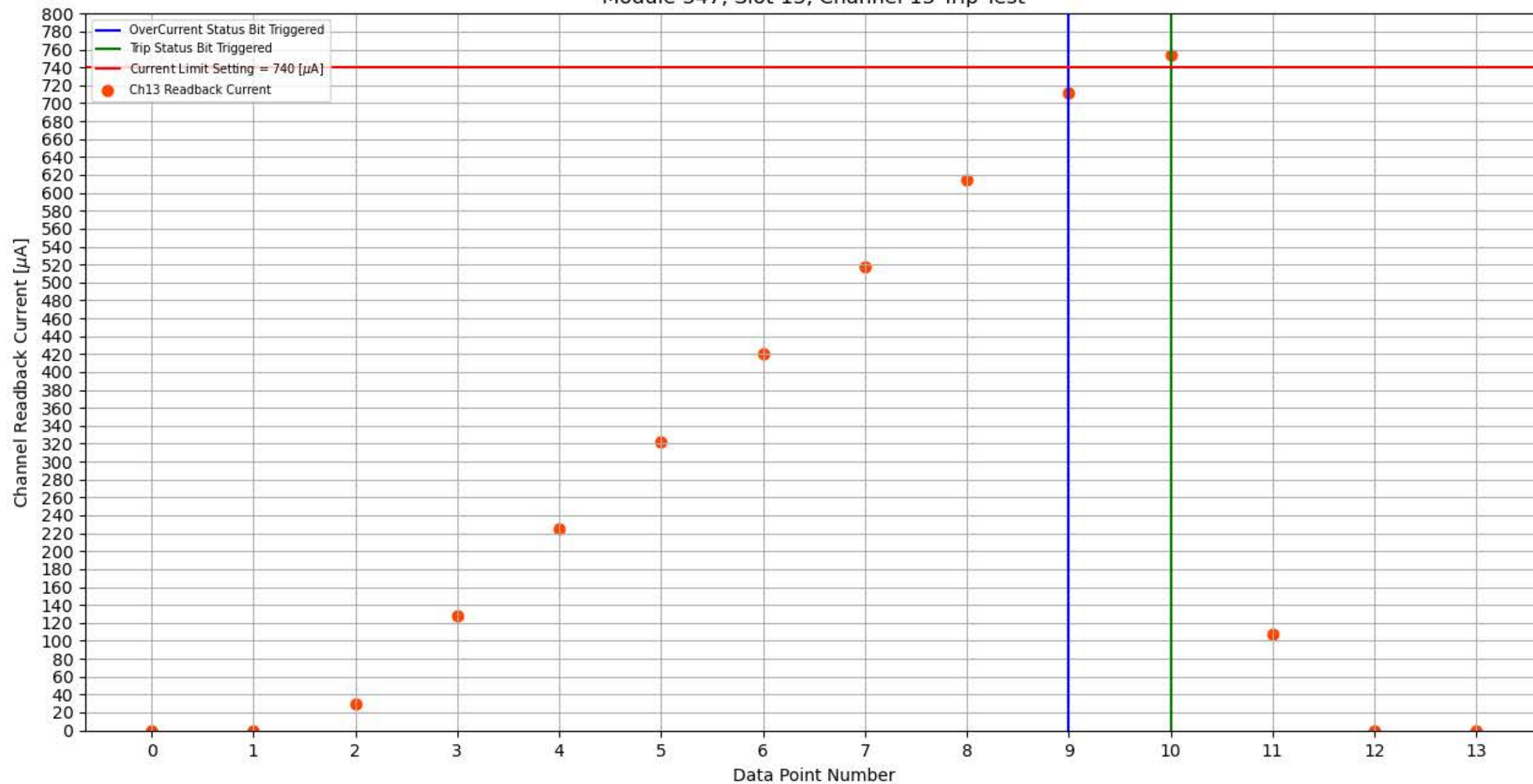
Module 347, Slot 13, Channel 13 Trip Test
