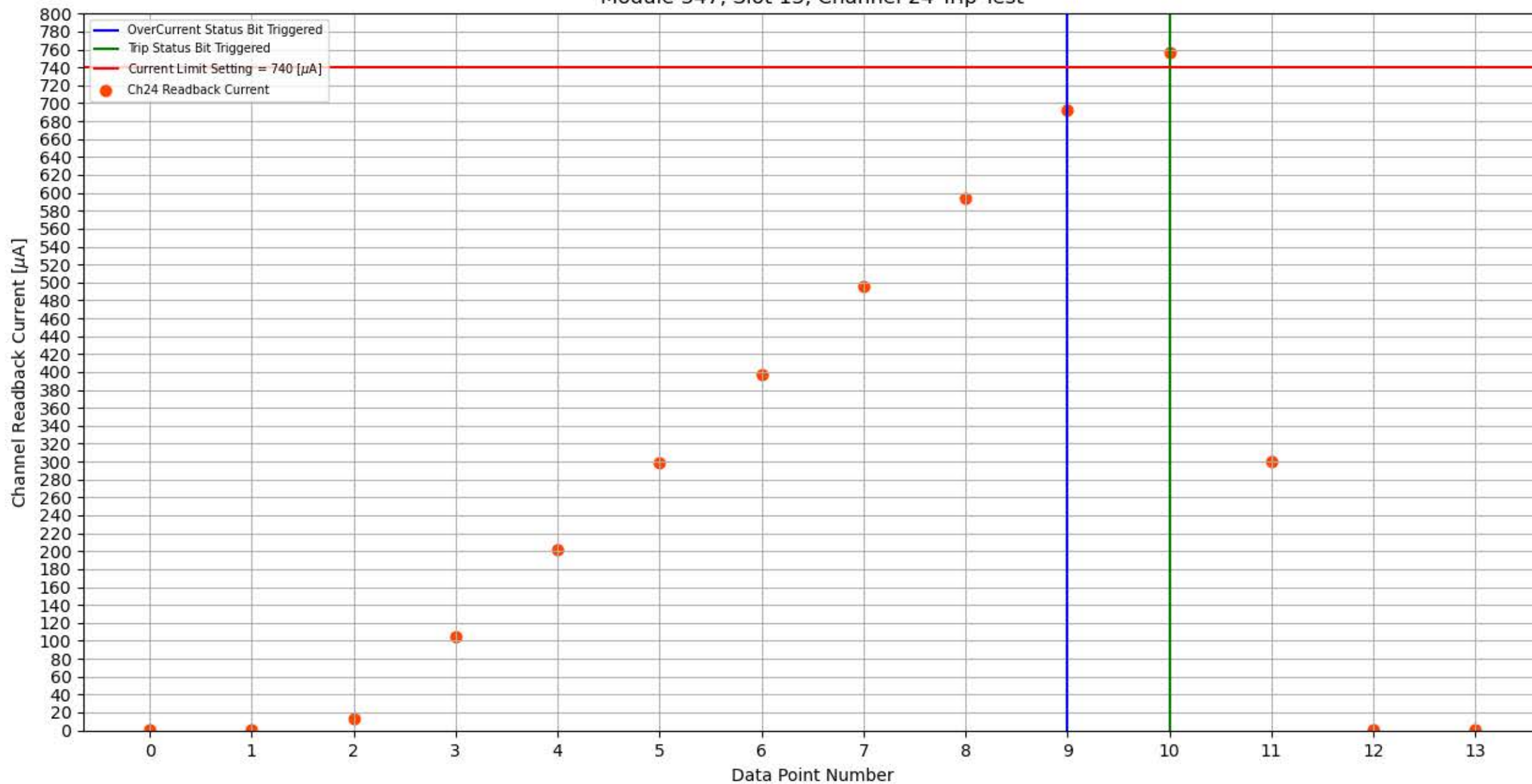
Module 347, Slot 13, Channel 24 Trip Test
