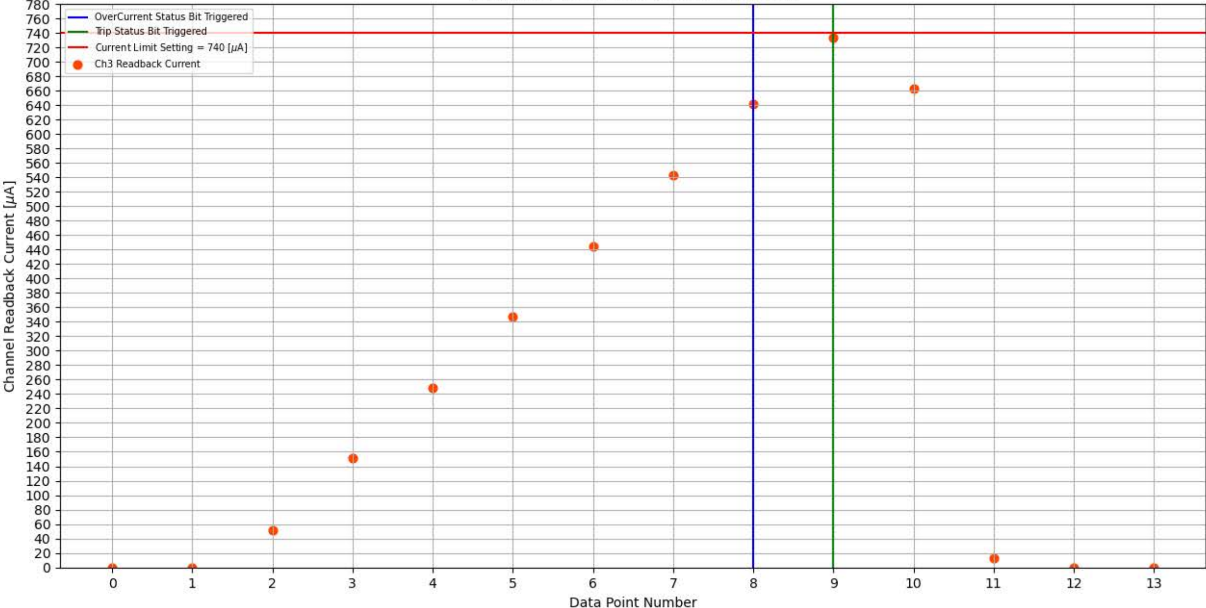
Module 347, Slot 13, Channel 3 Trip Test
