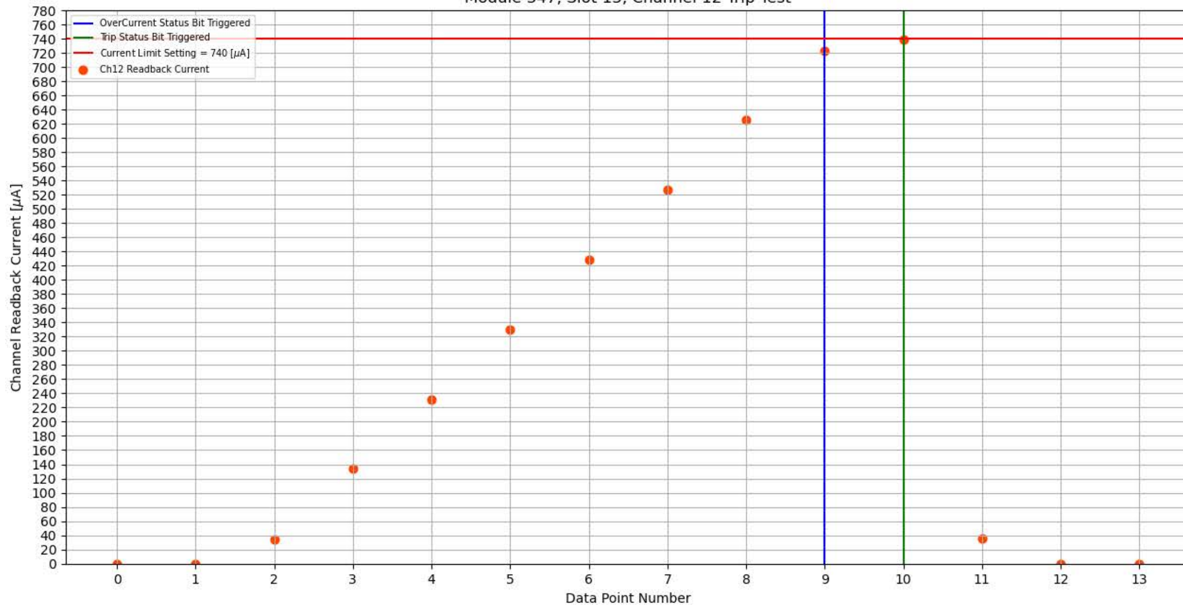
Module 347, Slot 13, Channel 12 Trip Test
