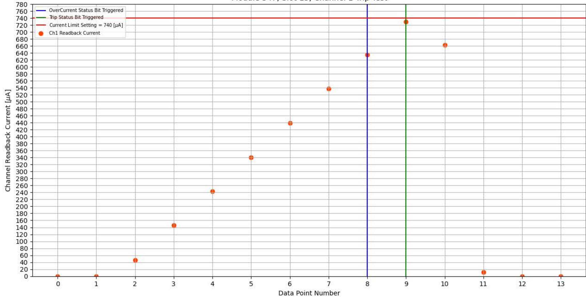
Module 347, Slot 13, Channel 1 Trip Test
