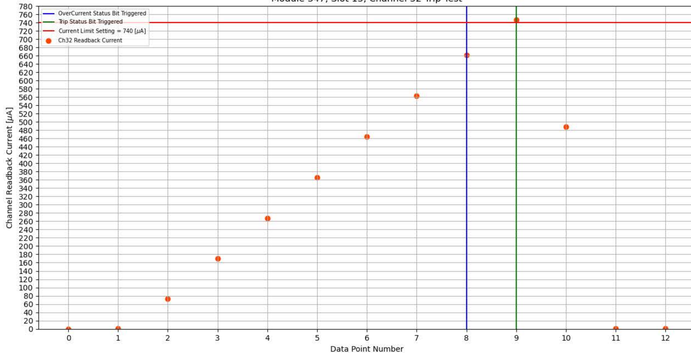
Module 347, Slot 13, Channel 32 Trip Test
