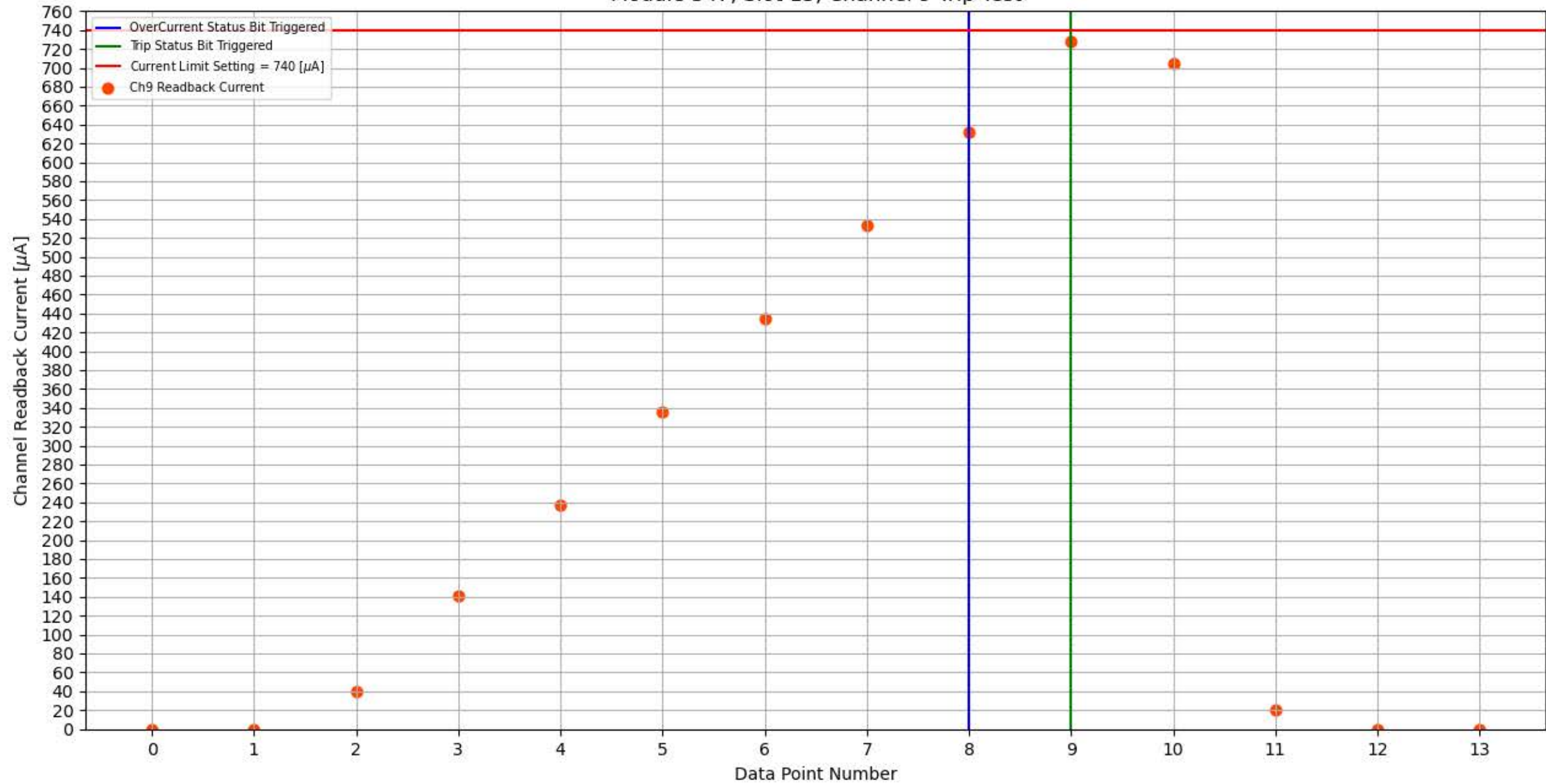
Module 347, Slot 13, Channel 9 Trip Test
