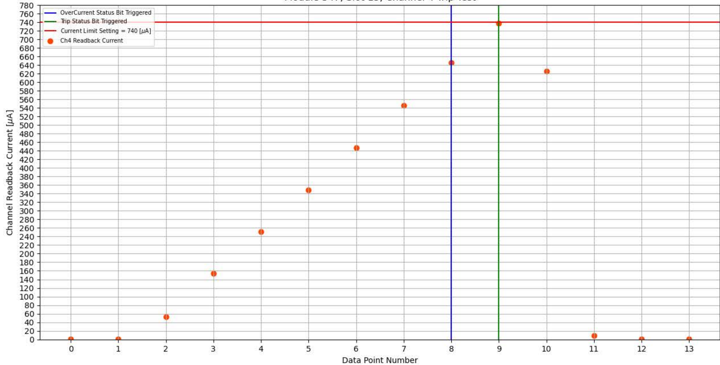
Module 347, Slot 13, Channel 4 Trip Test
