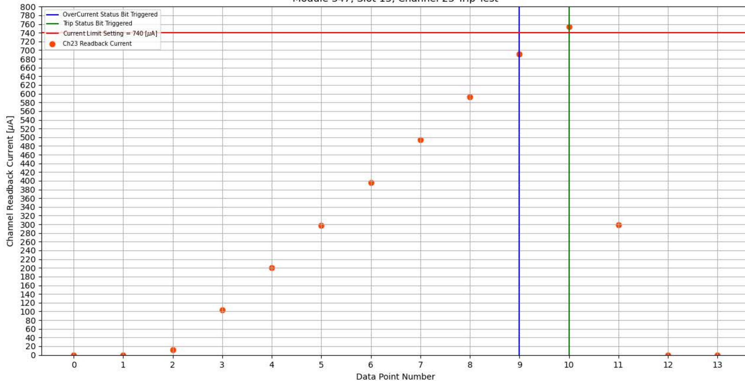
Module 347, Slot 13, Channel 23 Trip Test
