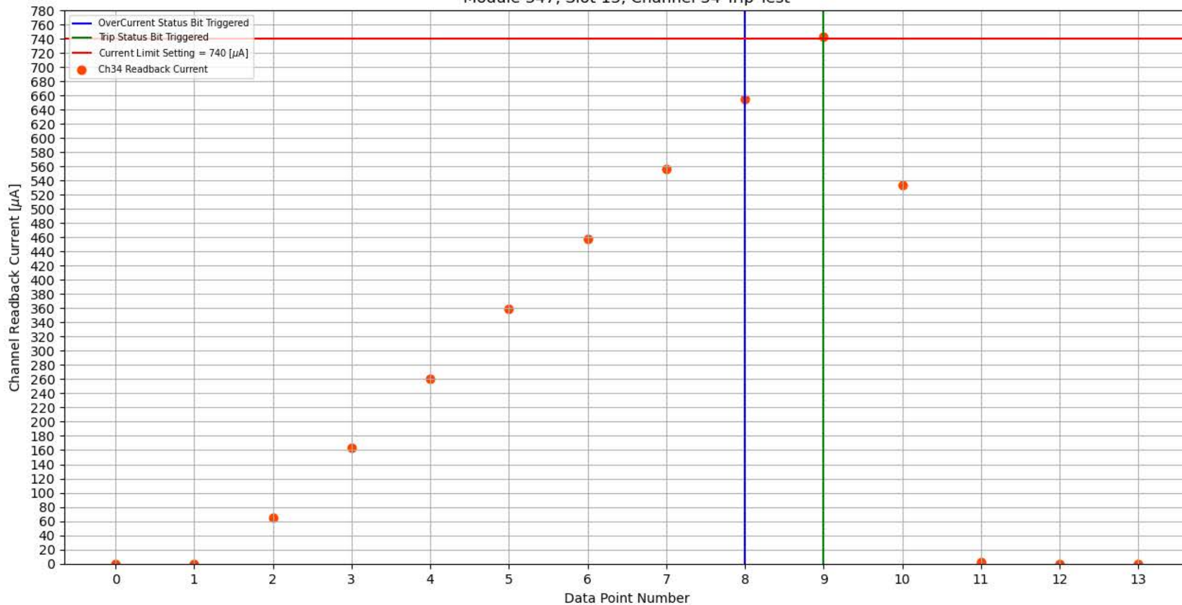
Module 347, Slot 13, Channel 34 Trip Test
