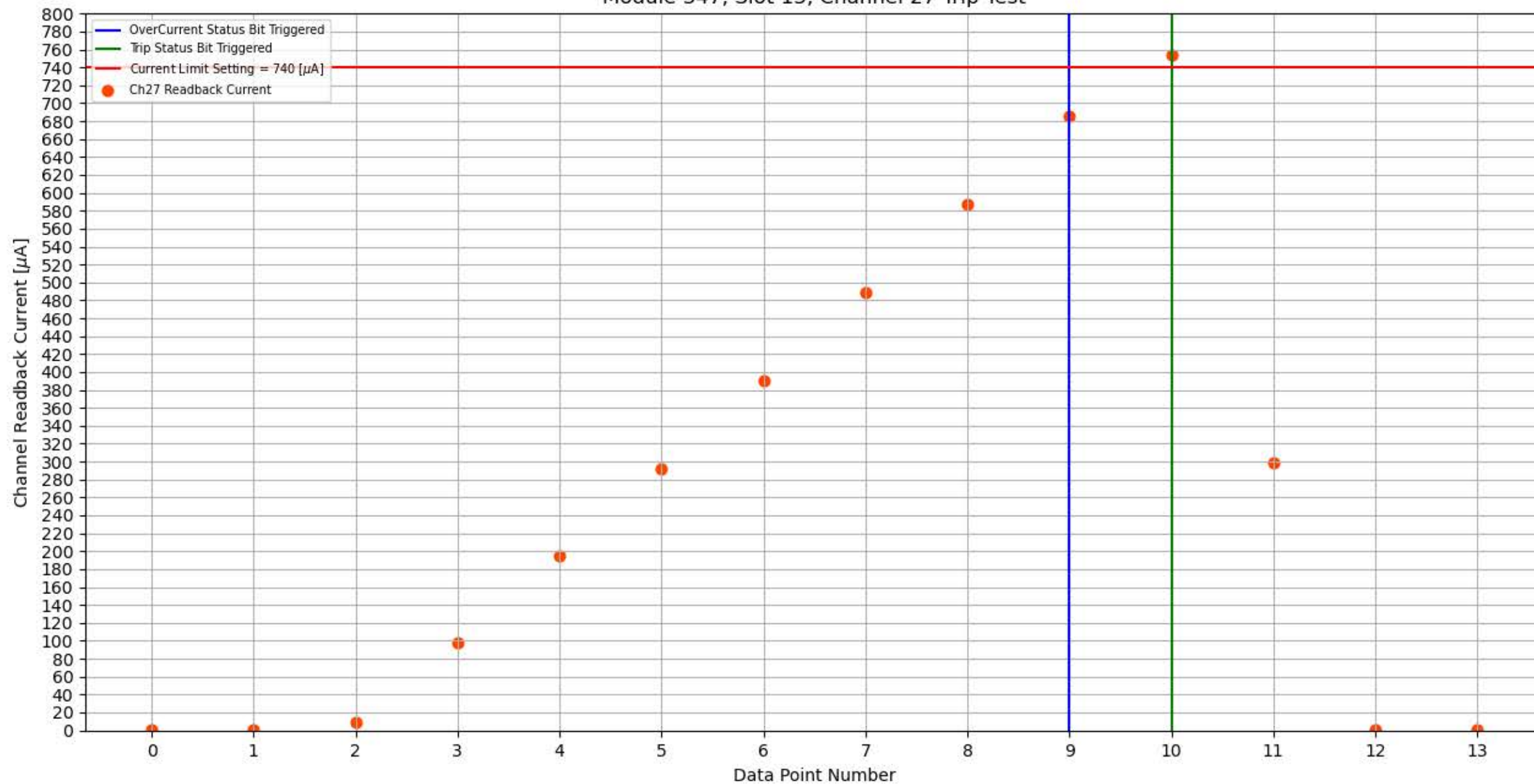
Module 347, Slot 13, Channel 27 Trip Test
