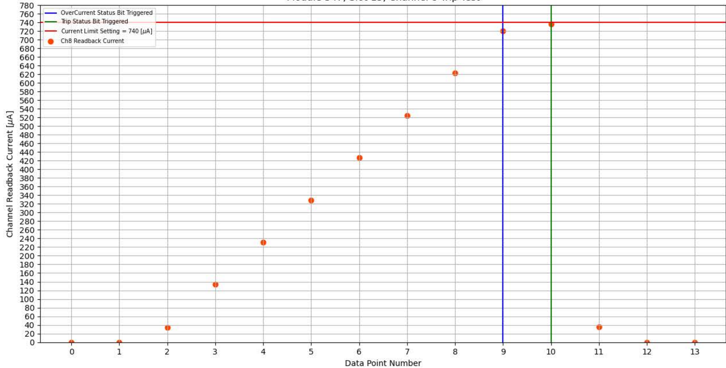
Module 347, Slot 13, Channel 8 Trip Test
