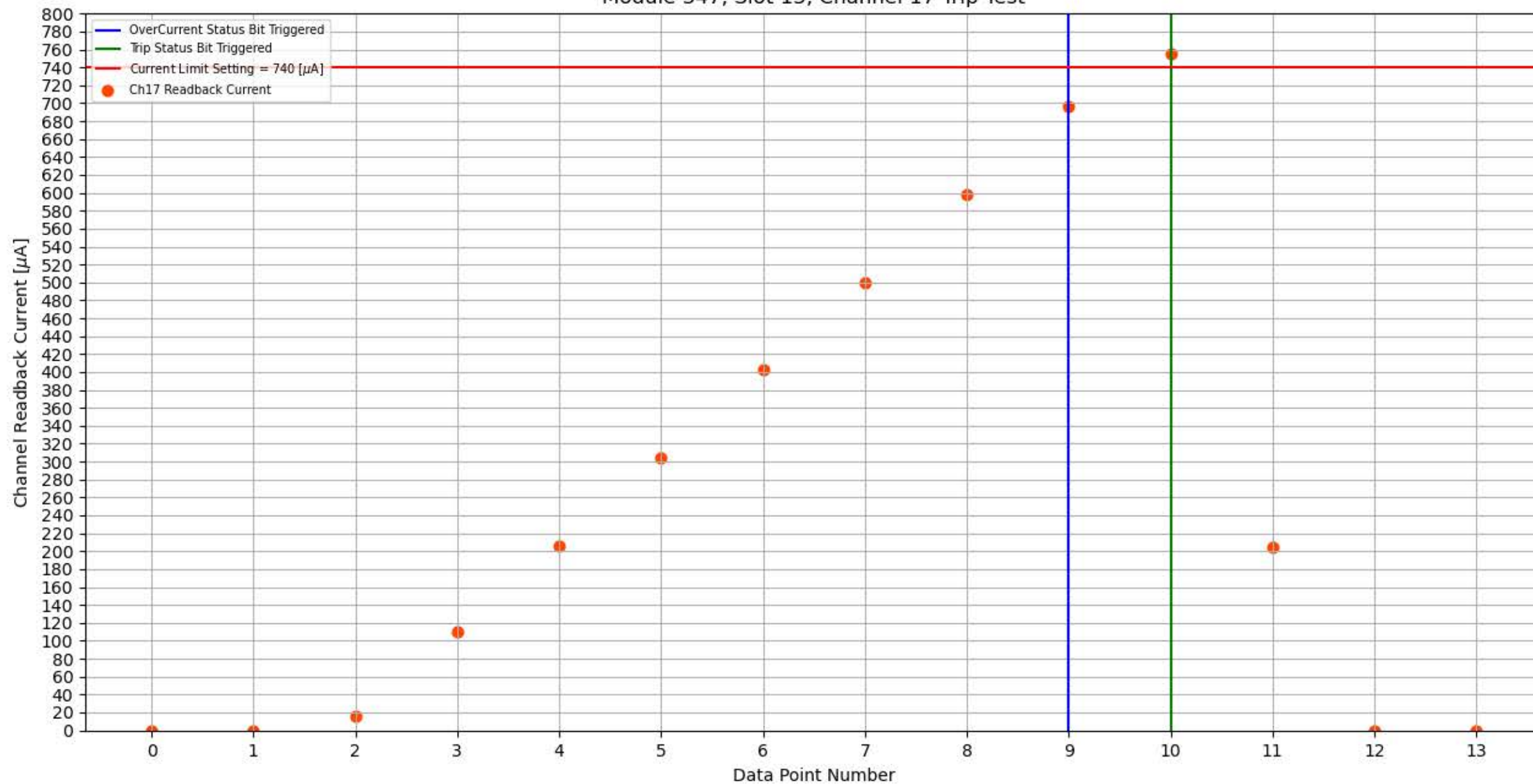
Module 347, Slot 13, Channel 17 Trip Test
