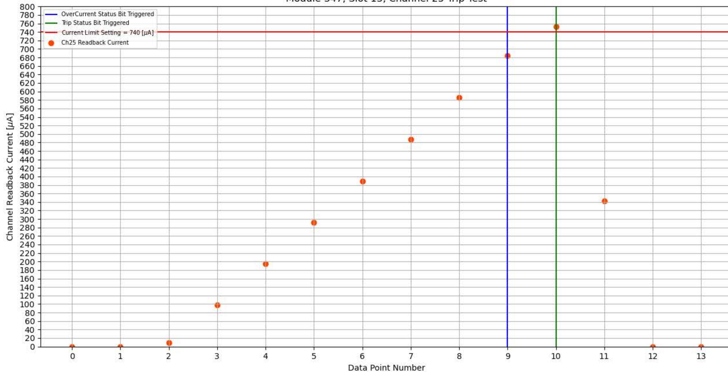
Module 347, Slot 13, Channel 25 Trip Test
