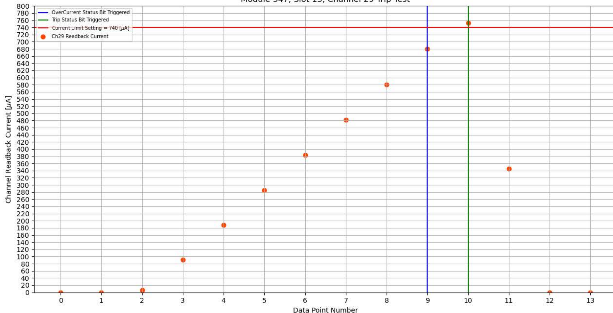
Module 347, Slot 13, Channel 29 Trip Test
