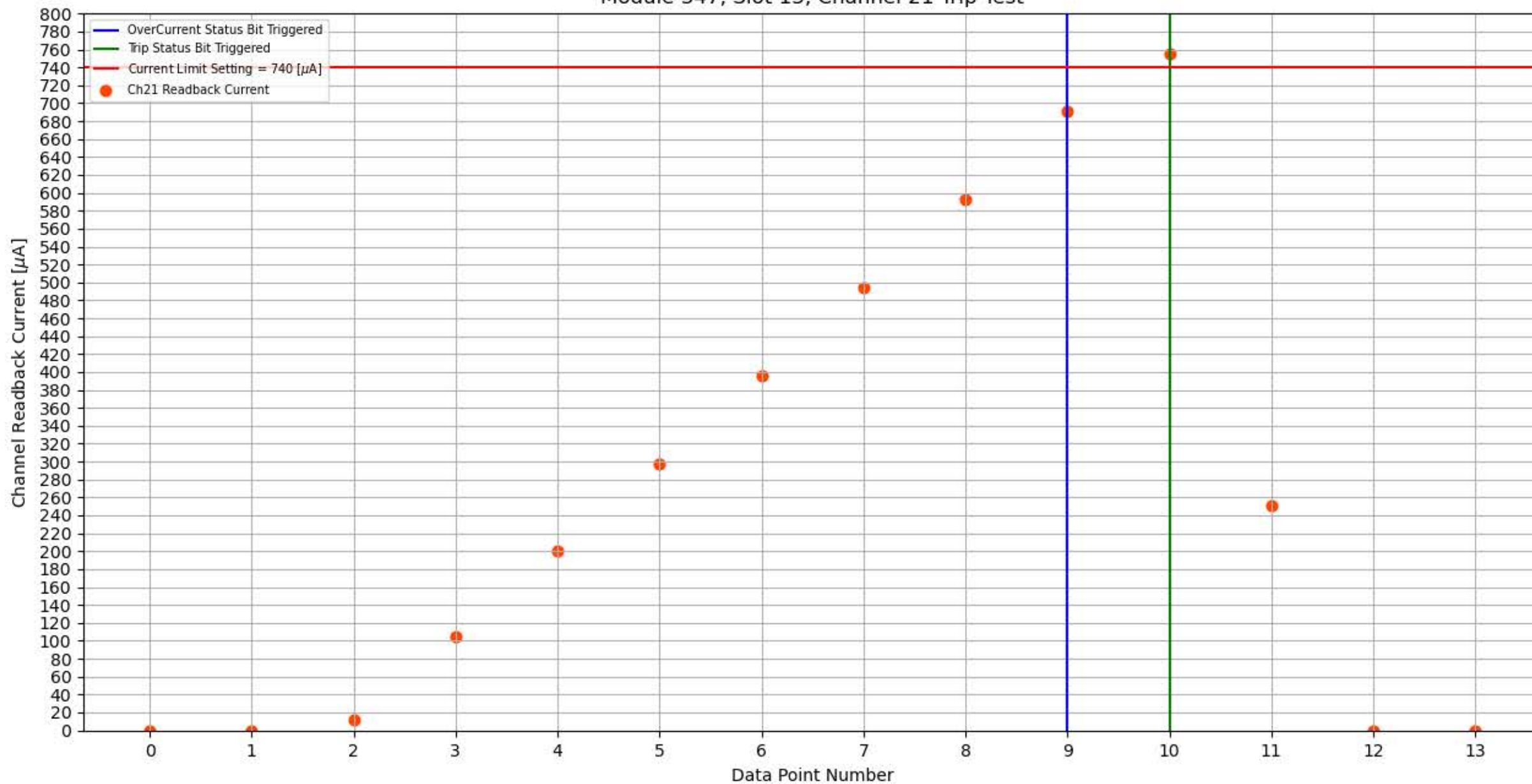
Module 347, Slot 13, Channel 21 Trip Test
