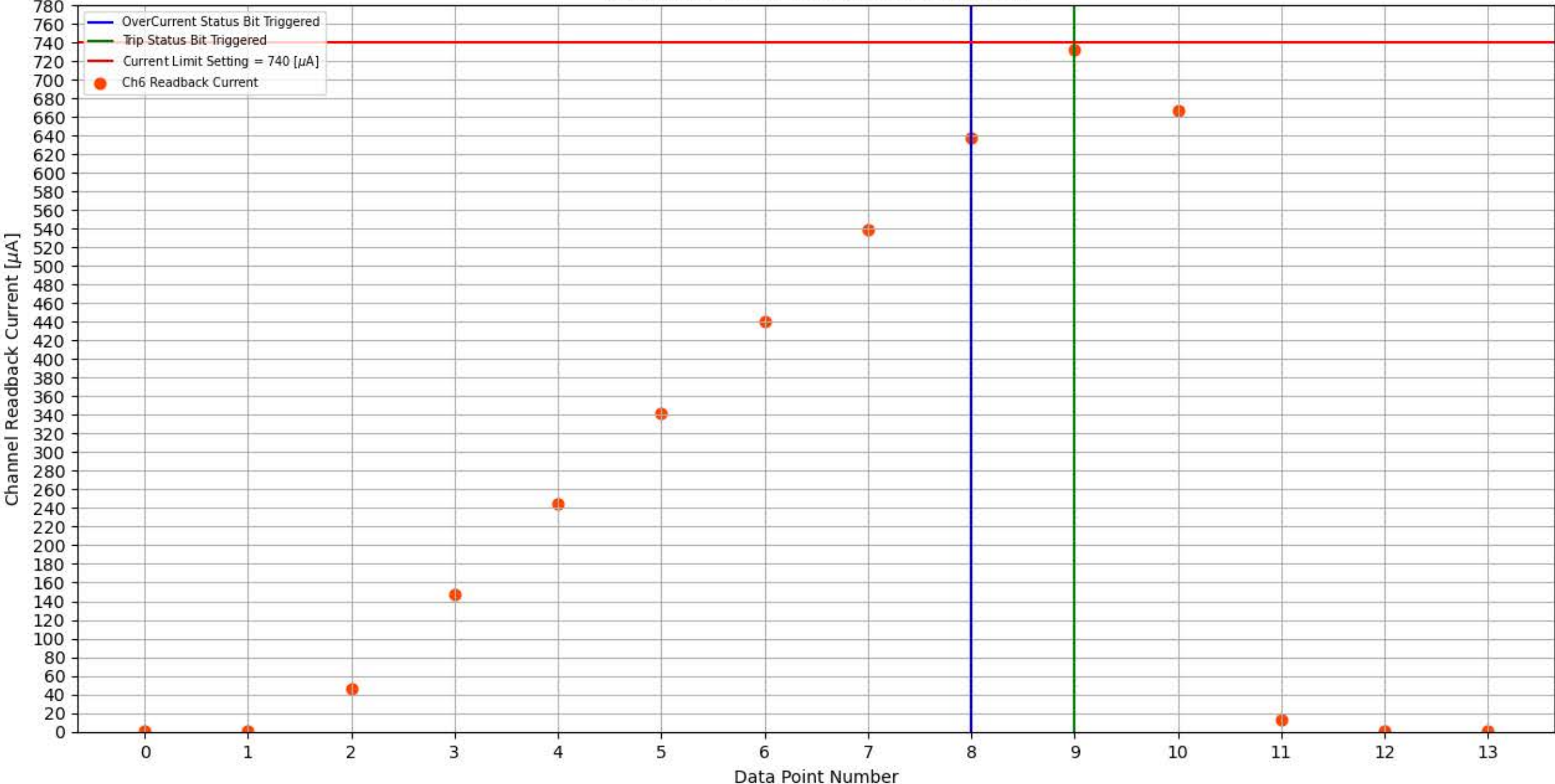
Module 347, Slot 13, Channel 6 Trip Test
