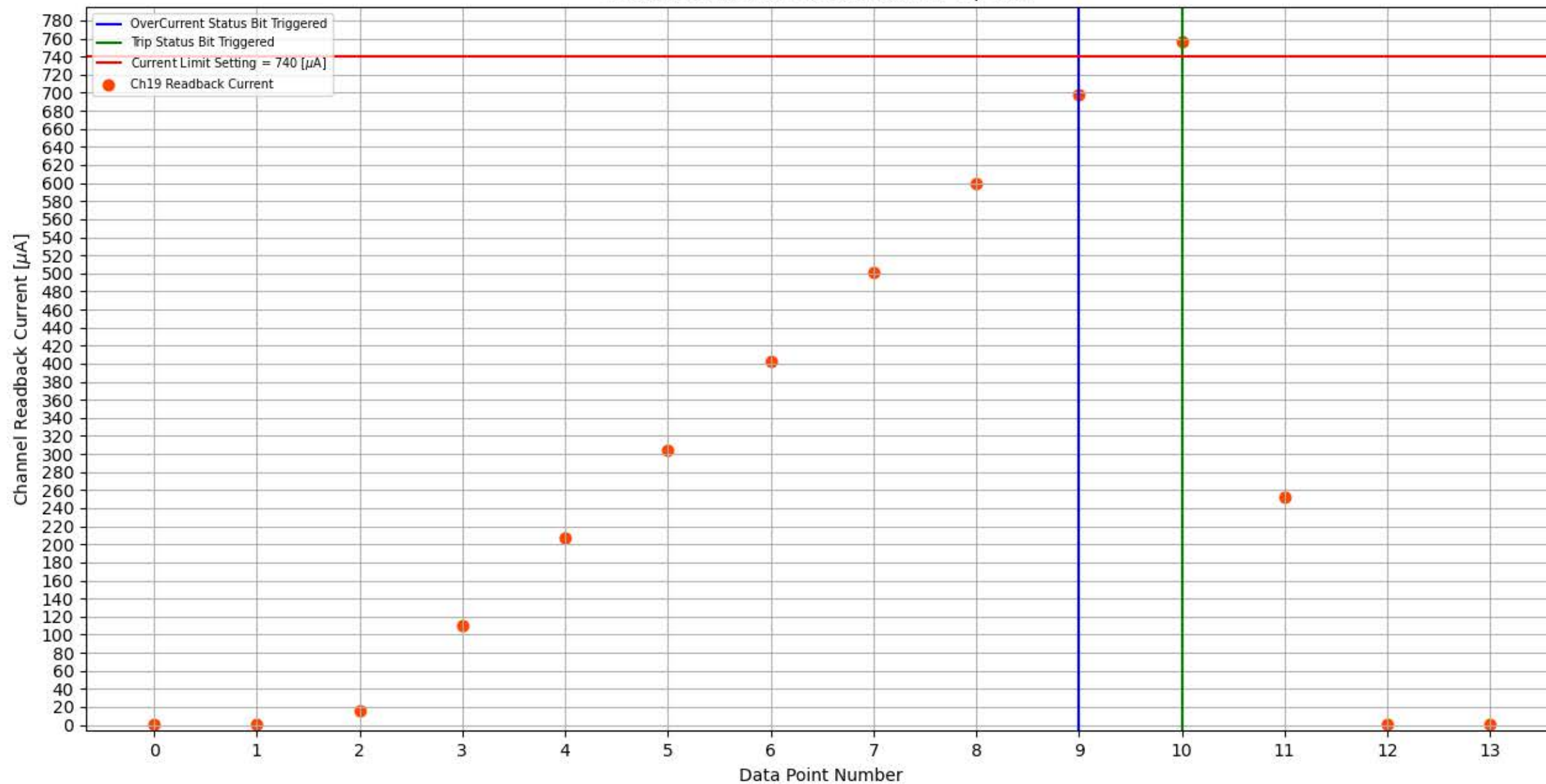
Module 347, Slot 13, Channel 19 Trip Test
