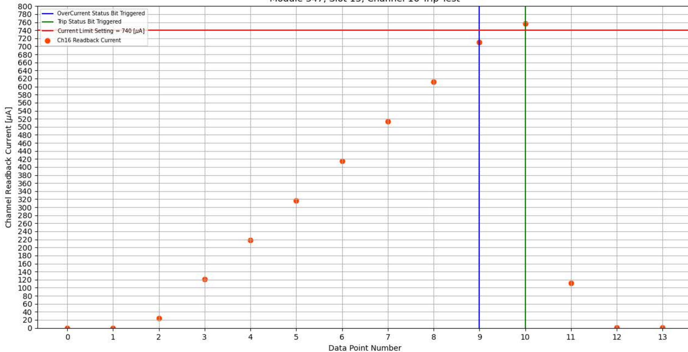
Module 347, Slot 13, Channel 16 Trip Test
