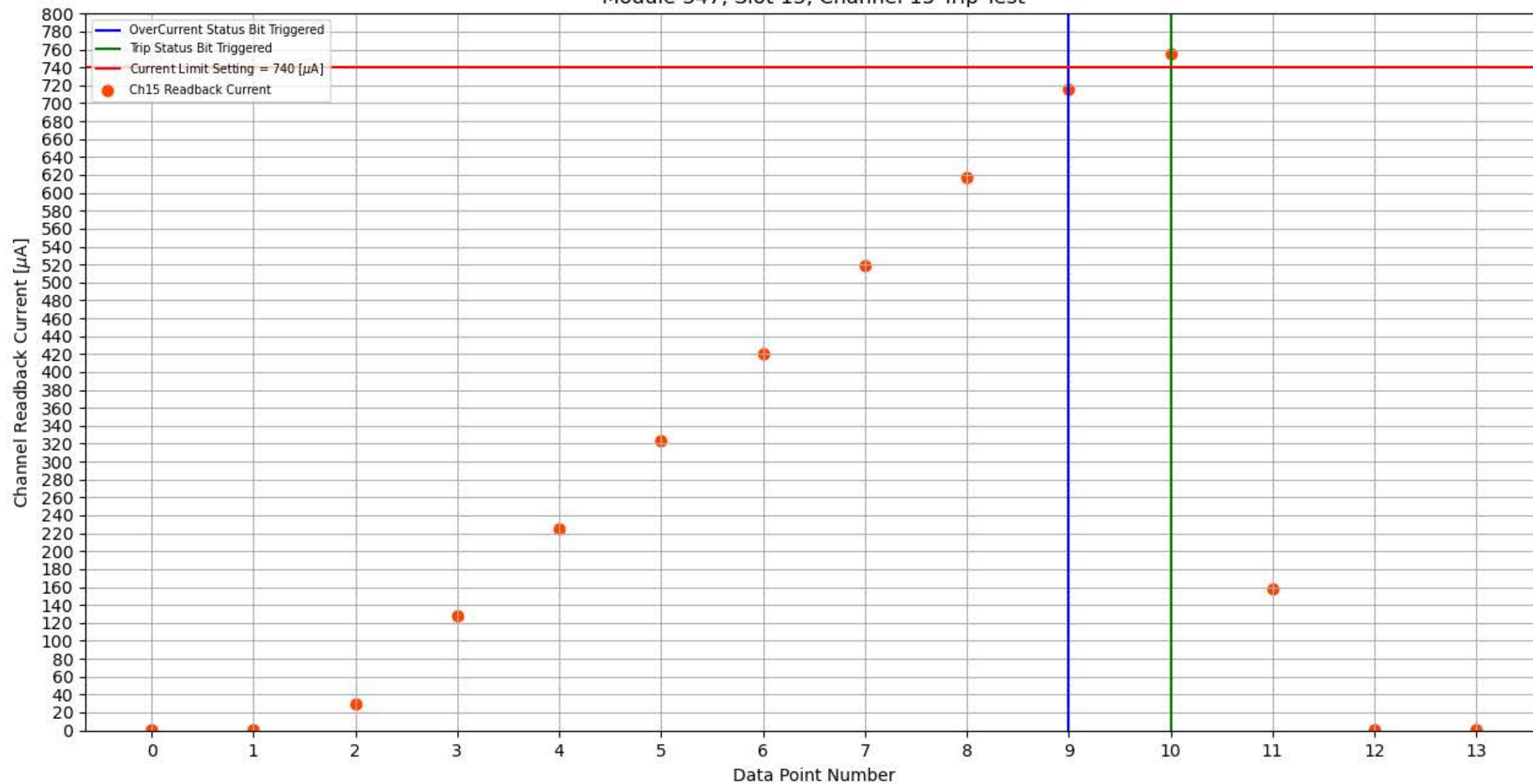
Module 347, Slot 13, Channel 15 Trip Test
