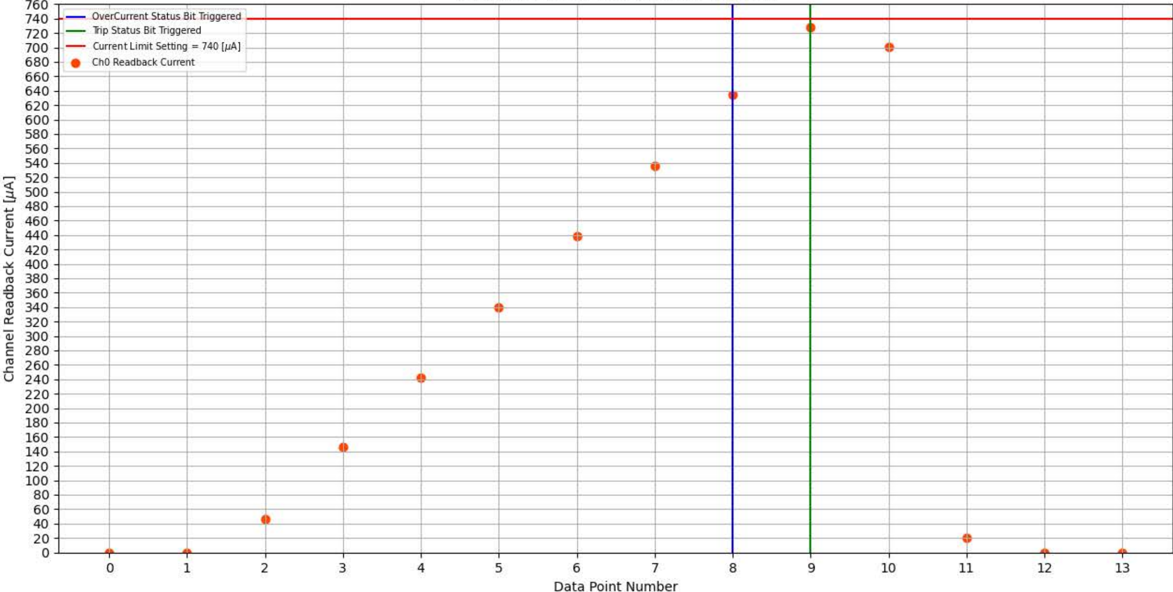
Module 347, Slot 13, Channel 0 Trip Test
