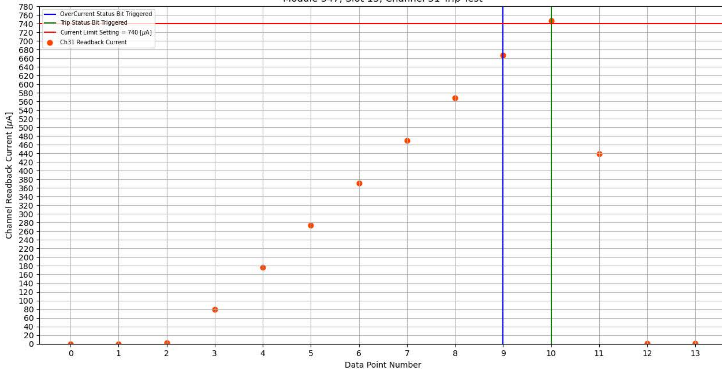
Module 347, Slot 13, Channel 31 Trip Test
