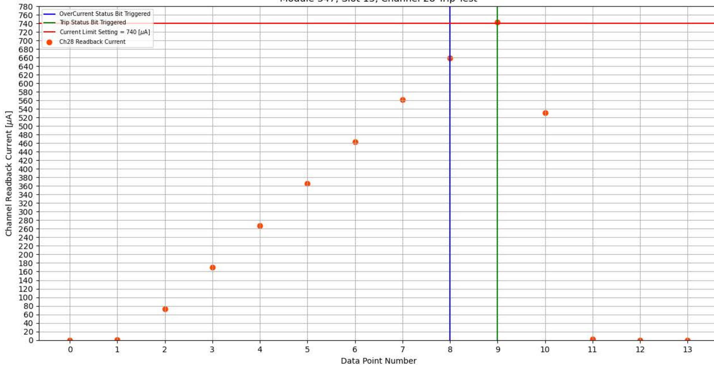
Module 347, Slot 13, Channel 28 Trip Test
