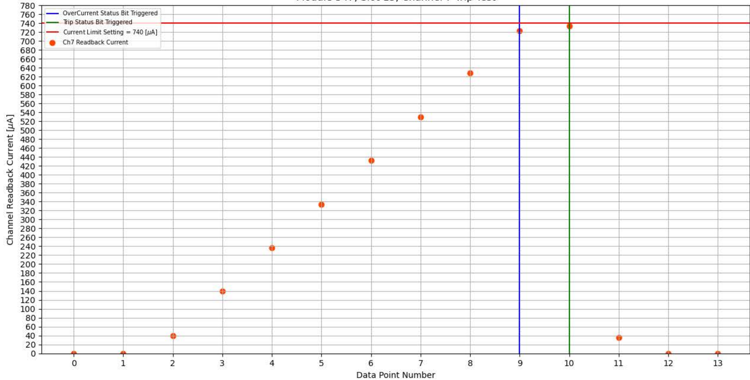
Module 347, Slot 13, Channel 7 Trip Test
